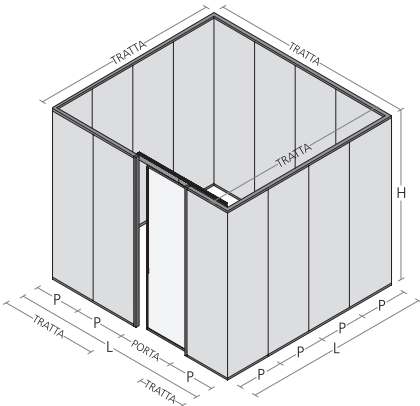
Anta scorrevole / Sliding door
