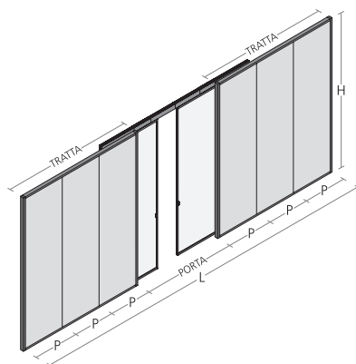
Anta scorrevole / Sliding door
