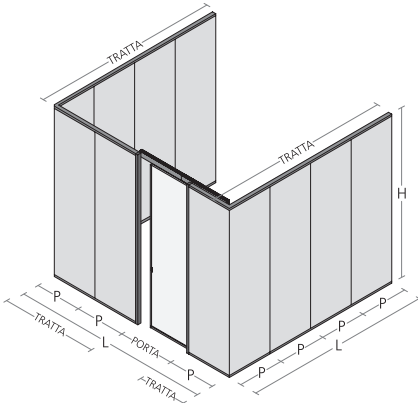
Anta scorrevole / Sliding door
