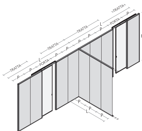
Anta scorrevole / Sliding door
