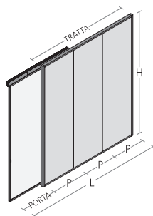
Anta scorrevole / Sliding door
