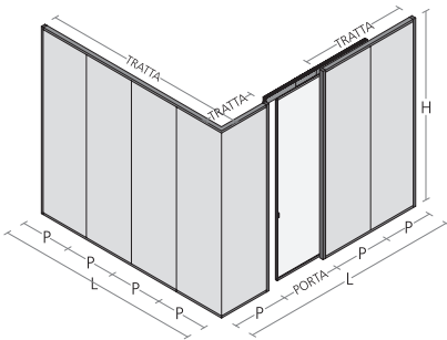
Anta scorrevole / Sliding door
