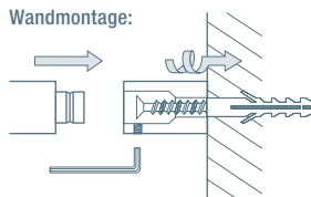
Wandmontage:
