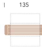
art. NKPSC porta sapone in ceramica ceramic soap holder porte-savon céramique Seifenschale aus Keramik dim. 13,5 x 9 cm
