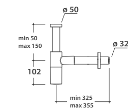
Siphon 1"1/4, weight: 1,16 kg Siphon schwarz matt 1"1/4, weight: 1,16 kg
