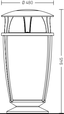
Idesia 2277.001 T
