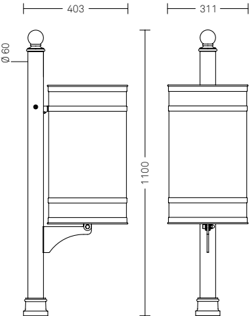
Melia 2275.000 C1 M 2275.100 C2 M
