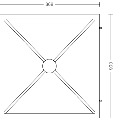
Melia – pannello 9525.439.030
