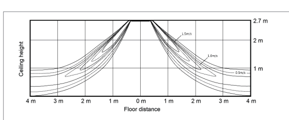
Heating Air Velocity distribution
