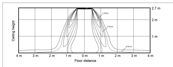
Cooling Air Velocity distribution
