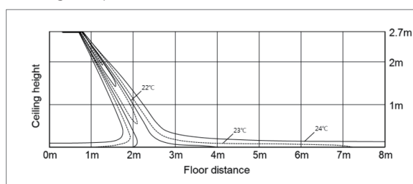
Cooling temperature distribution
