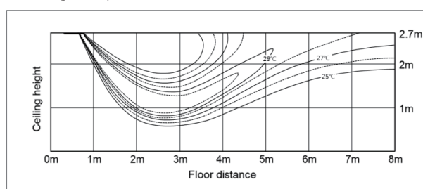
Heating temperature distribution
