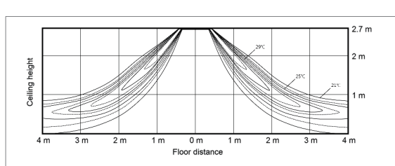
Heating temperature distribution
