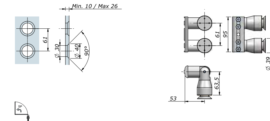
Cerniera verticale con doppia borchia svasata Vertical hinge with double countersunk boss
