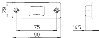
PI036 Controbordo in nylon nero
