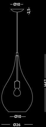
GIG1253.1L Sospensione / Hanging lamp vetro/glass Ø26 cm - cavo/cable 150 cm 1 E27 x max 70W 220-240V CE IP20 1m
