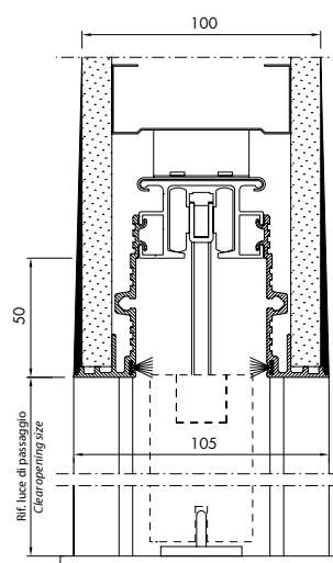
Parete in Cartongesso da 100 mm Plasterboard walls with thicknesses 100 mm
