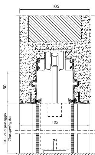
Parete in muratura da 105 mm Masonry walls with thicknesses 105 mm
