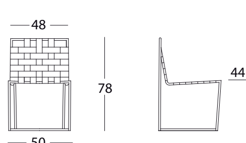
Sedia _ Chair
