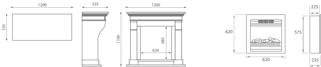
Kreta Suite Stufa Melini
