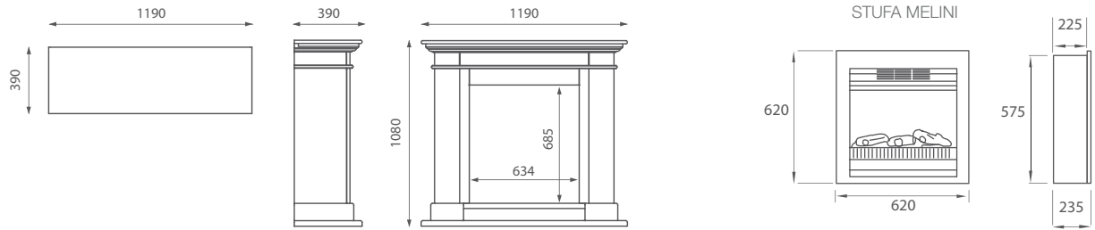
Kos Suite Stufa Melini
