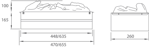
Mystic Fire 1720C Mystic Fire 1740C
