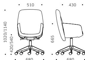
VIC6X / VIS6X
