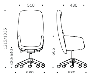
VIC8X / VIS8X
