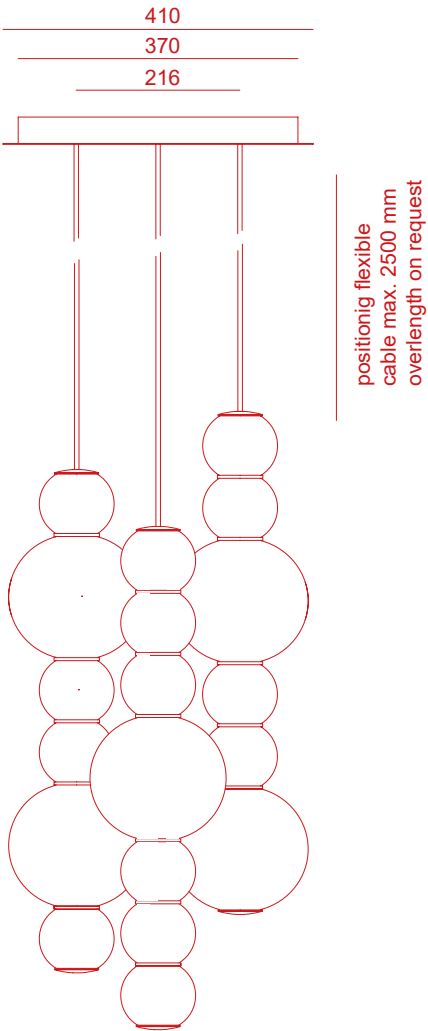
PEARLS DOUBLE Chandelier 3
