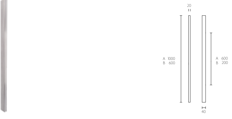
LSQ1075 massieve greep tbv houten, glazen of aluminium deuren doorgaande of paarsgewijze bevestiging | solid pull handle for timber, glass or aluminium doors bolt-through or back to back fixings
