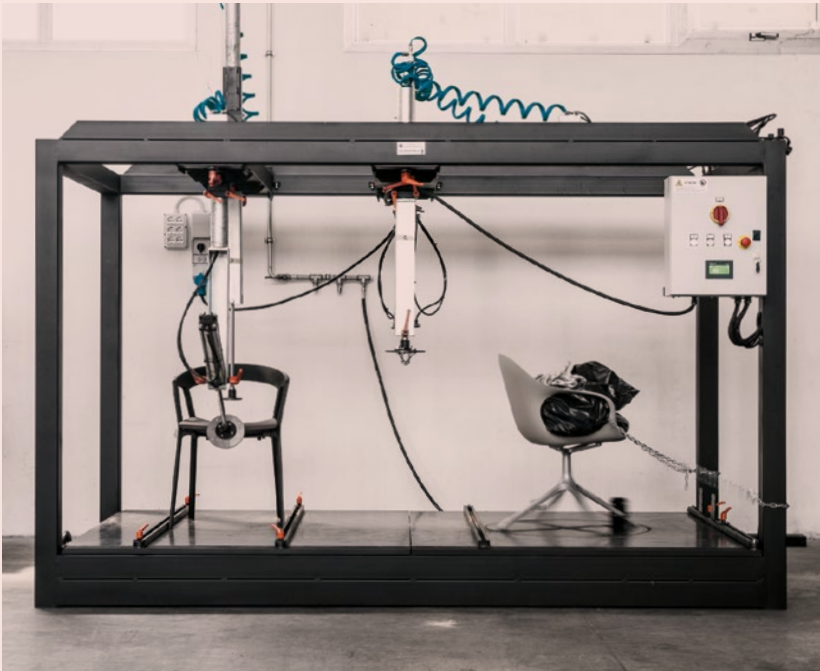
"Ercole" test machine
