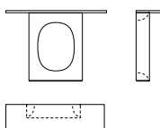
Console table L 140 P 35 H 94 cm W 55 1 / 8 " D 13 5 / 8 " H 37"
