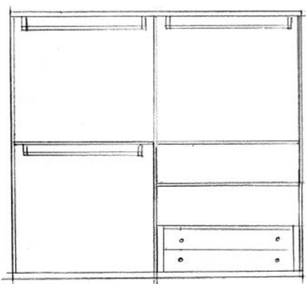
ART. ECLMC200 Michelangelo Armadio 2 ante scorrevoli 3 ripiani, 3 bastoni appendiabiti, 1 cassettiera 2 cassetti 2 sliding door wardrobe 3 shelves, 3 clothes rail, 1 drawers unit with 2 drawers
