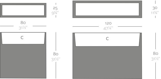
Wall 31 1/2" Wall 80 cm Wall 47 1/4" Wall 120 cm
