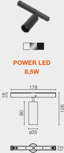
SPOT 150
