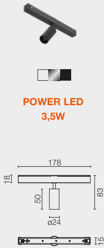
SPOT 120
