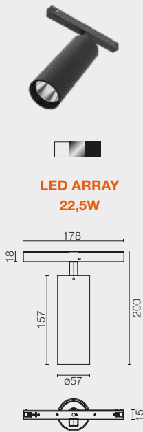
SPOT 150
