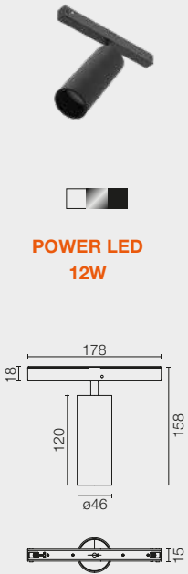
SPOT 120
