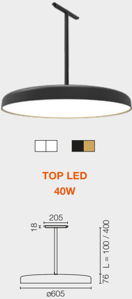
SUSPENSION PANEL 600
