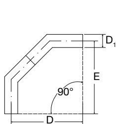
2 curve montate a 90° 2 bends mounted at 90°
