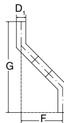
Spostamento 2 curve a 45° + elemento Displacement of 2 bends at 45° + element
