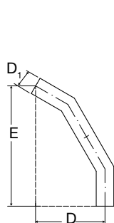
2 curve montate a 60° 2 bends mounted at 60°
