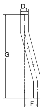
Spostamento 2 curve a 15° + elemento Displacement of 2 bends at 15° + element
