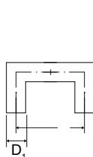
2 curve montate a 180° 2 bends mounted at 180°
