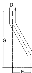
Spostamento 2 curve a 30° + elemento Displacement of 2 bends at 30° + element
