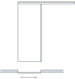
1 ANTA BINARIO AD 1 VIA A PARETE 1 DOOR 1-WAY RUNNER WALL ASSEMBLY
