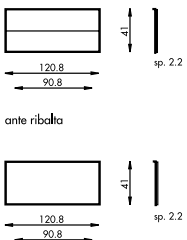
cassetti_drawers
