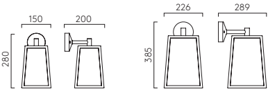
CALVI WALL 215
