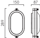
MALIBU OVAL
