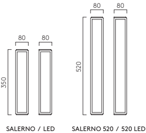
SALERNO / LED
