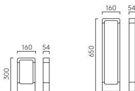
NAPIER BOLLARD 300
