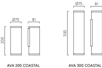
AVA 200 COASTAL
