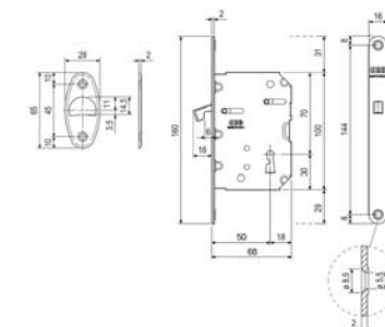
SD505 set rosette incasso foro chiave con frontale + serratura sliding door handle set key hole with flush pull hole + lock
