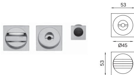
2186/S set rosette incasso con nottolino q. 8 mm con frontale sliding door handle set with turn and release 8 mm square spindle and flush pull hole
