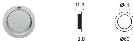
SD500 rosetta incasso sliding door handle
