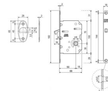
SD506 set rosette incasso con nottolino q. 8 mm con frontale +serratura sliding door handle set with turn and release 8 mm square spindle with flush pull hole + lock
