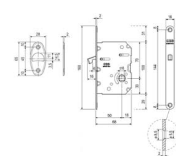
2194/SE108 set rosette incasso con nottolino q.8 mm con frontale + serratura sliding door handle set with turn and release 8 mm square spindle with flush pull hole + lock
