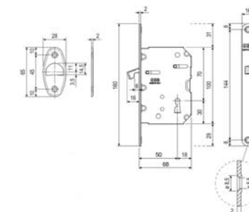
2185/SE107 set rosette incasso foro chiave con frontale + serratura sliding door handle set key hole with flush pull hole + lock
