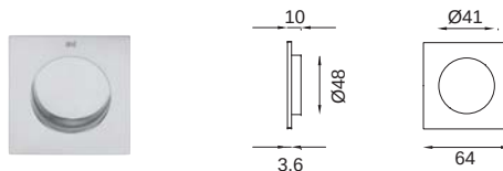
SD220 rosetta incasso sliding door handle
