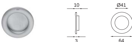
SD200 rosetta incasso sliding door handle
