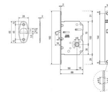
2186/SE108 set rosette incasso con nottolino q.8 mm con frontale + serratura sliding door handle set with turn and release 8 mm square spindle with flush pull hole + lock
