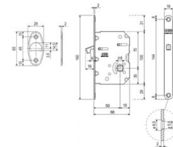
SD226 set rosette incasso con nottolino q.8 mm con frontale + serratura sliding door handle set with turn and release 8 mm square spindle with flush pull hole + lock
