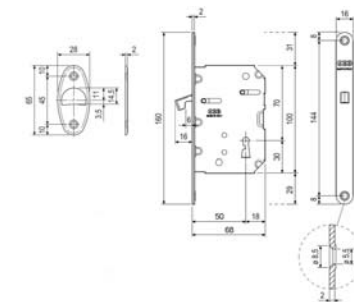
SD225 set rosette incasso foro chiave con frontale + serratura sliding door handle set key hole with flush pull hole + lock
