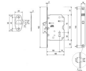
2193/SE107 set rosette incasso foro chiave con frontale + serratura sliding door handle set key hole with flush pull hole + lock
