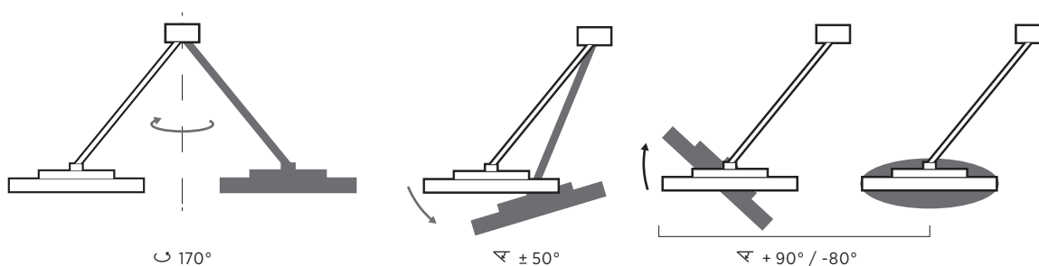
SIGN DIVA DANCER - POSSIBLE ADJUSTMENTS
