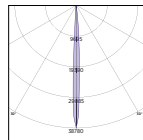
SUPER SPOT 125 I max : 26 630 cd/klm (53 260 cd abs.) FWHM: 2x 3,7°
