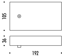
CEILING ROSE
