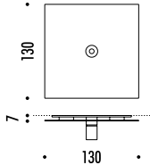
CEILING ROSE
