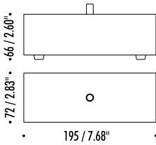
DRIVER
