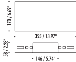
WALL ROSE
