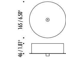
CEILING ROSE
