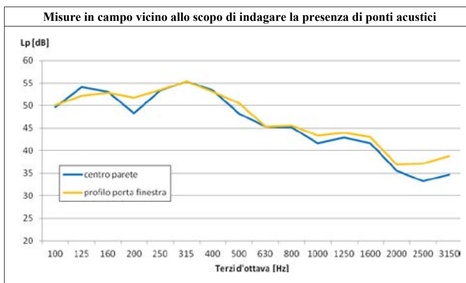
Fig. 6 – misure in campo vicino
