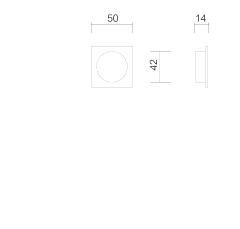
Art. 2440 Nicchia quadrata d/50 liscia Flush handle d/50 plain
