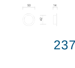
Art. 2420 Nicchia tonda d/50 liscia Flush handle rounded d/50 plain
