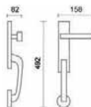
Art. 4129 Set America Set America
