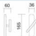
Art. 2412 Cremonese Window handle
