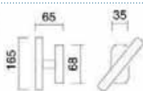
Art. 0032 Cremonese Window Handle
