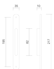
Art. 617 Liscia cieca c/foro Flush handle w/hole
