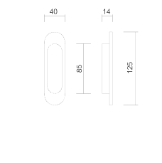
Art. 3543/P Nicchia a/ribalta cieca c/foro Flush handle w/hole
