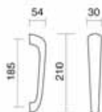
Art. 3785 Maniglione Princess Pull handle Princess
