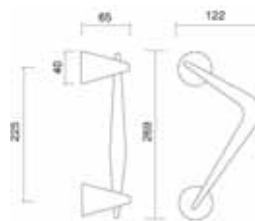
Art. 0110 Maniglione Boomerang Pull handle Boomerang
