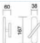
Art. 1802 Cremonese Window handle
