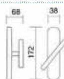
Art. 0012 Cremonese Window Handle
