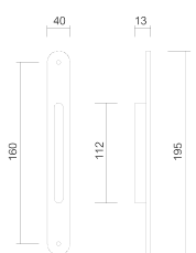
Art. 618 Nicchia cieca c/foro Flush handle w/hole
