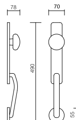
Art. 4141 Set America Set America
