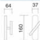
Art. 2792 Cremonese Window handle
