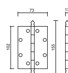
Art. 132 Cerniera piccola Small Hinge
