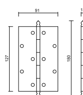
Art. 131 Cerniera grande Big Hinge
