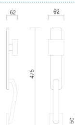
Art. 4139 Set America Set America
