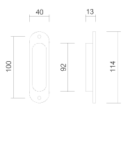
Art. 3543 Liscia cieca Flush handle w/hole
