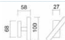
Art. 2953 Martellina Window handle
