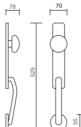
Art. 4140 Set America Set America
