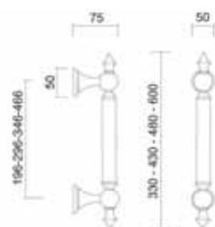
Art. 0200 Maniglione Manila Pull handle Manila
