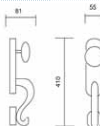
Art. 4109 Set America Set America
