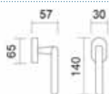
Art. 2862 Cremonese Window handle
