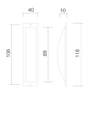
Art. 616 Nicchia cieca c/foro Flush handle w/hole
