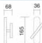
Art. 0022 Cremonese Window handle
