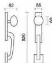
Art. 4125 Set America Set America
