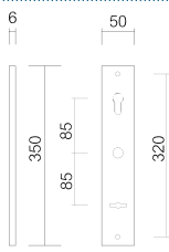
Art. P 3540 YDM Placca sp. Quadrata Special plate Quadrata
