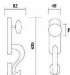
Art. 4102 Set America Set America
