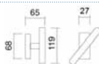
Art. 3073 Martellina Window handle
