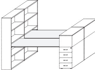
nr.2 scrivanie su profcase e mobile portante nr. 2 desks desk on profcase and supporting cabinet
