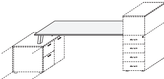
scrivania su servente e mobile portante desk on service unit and supporting cabinet
