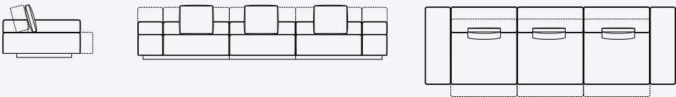
Divano 3 posti Three-seater sofa L.2760 H. 560 – 770 P. 1200 – 1380 W. 107 3/4” H 22” – 30¾” D. 47¼” – 52¼”
