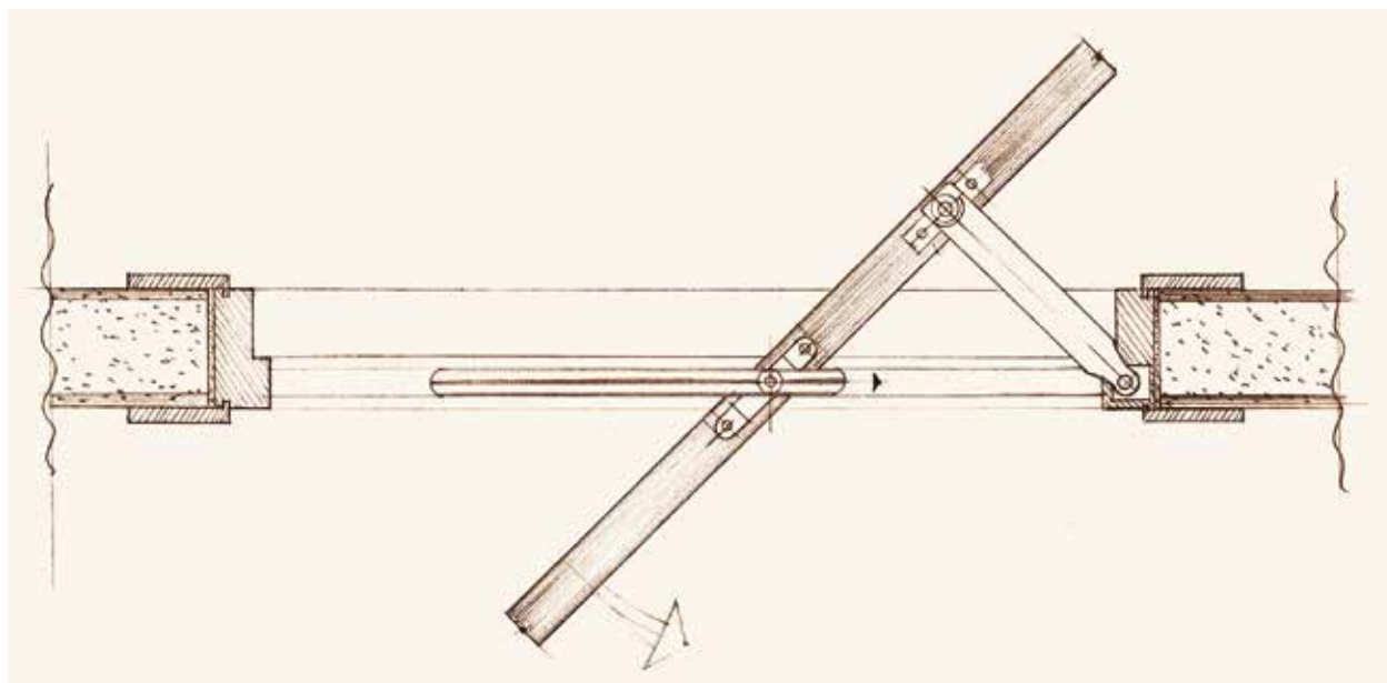
Porta scorrevole rototraslante - Pivot sliding mechanism
