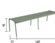
BENCH BANK Steel Stahl 14.5 kg
