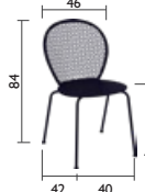
Steel Stahl 12 kg
