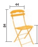
CHAIR STUHL Steel Stahl 5.8 kg
