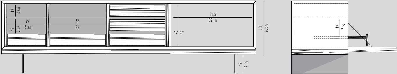
CONTENITORE “DINING” CM 252X60 H72 CON 1 ANTA E 1 VANO PASSANTE | “DINING” SIDEBOARD CM 252X60 H72 WITH 1 DOOR AND 1 OPEN SECTION
