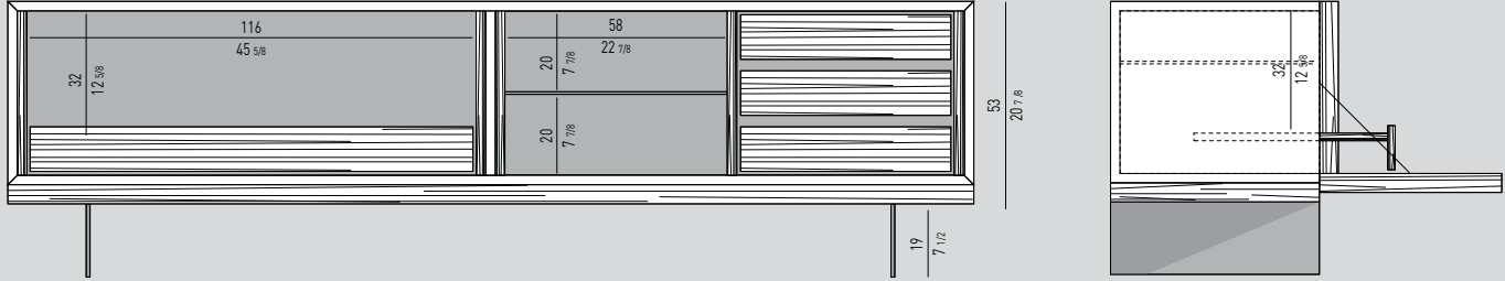
CONTENITORE “DINING” CM 252X60 H72 CON 2 ANTE | “DINING” SIDEBOARD CM 252X60 H72 WITH 2 DOORS
