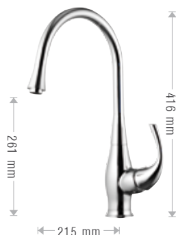
571/PN PLUTO Miscelatore monocomando lavello bocca girevole. Single-lever sink mixer with swivel spout.
