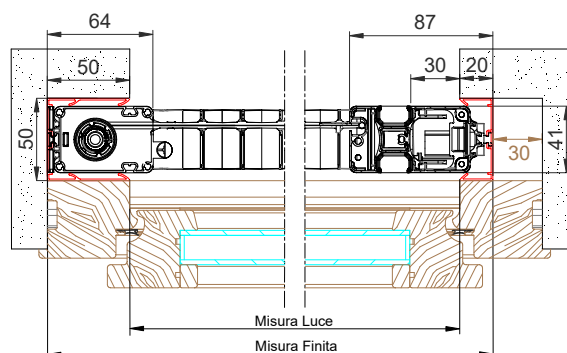
■ BORA INCAS MIDI 50/20
