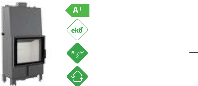
LUCY PW 12 513x706x1384/1413x452
