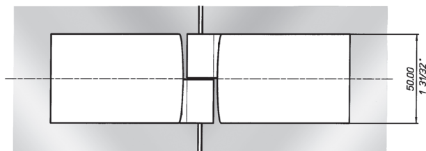
GAHA1G16D Vetro - Vetro Glass to Glass
