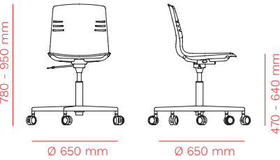
MIA SWIVEL CHAIR art. 3300
