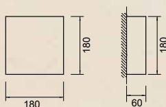
DIVETRO 18 Led 17W – 230Vac – 3000K CE Peso / Weight 0,75 kg
