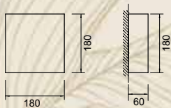
COLORVETRO 18 Led 17W – 230Vac – 3000K CE Peso / Weight 0,8 kg
