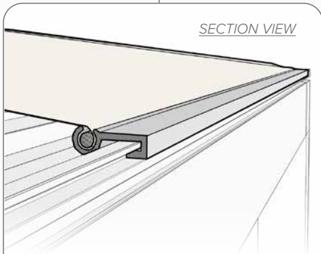
PERIMETER FASTENING OF THE ROOF COVER
