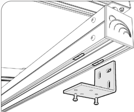
WALL-TYPE FASTENING SYSTEM
