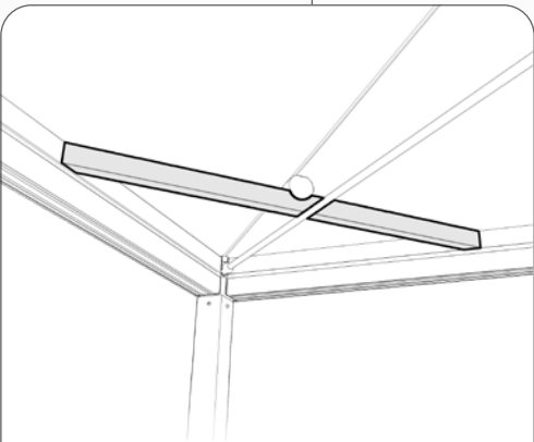
CORNER BRACINGS SUPPLIED ON STRUCTURES GREATER THAN 450 cm WIDE
