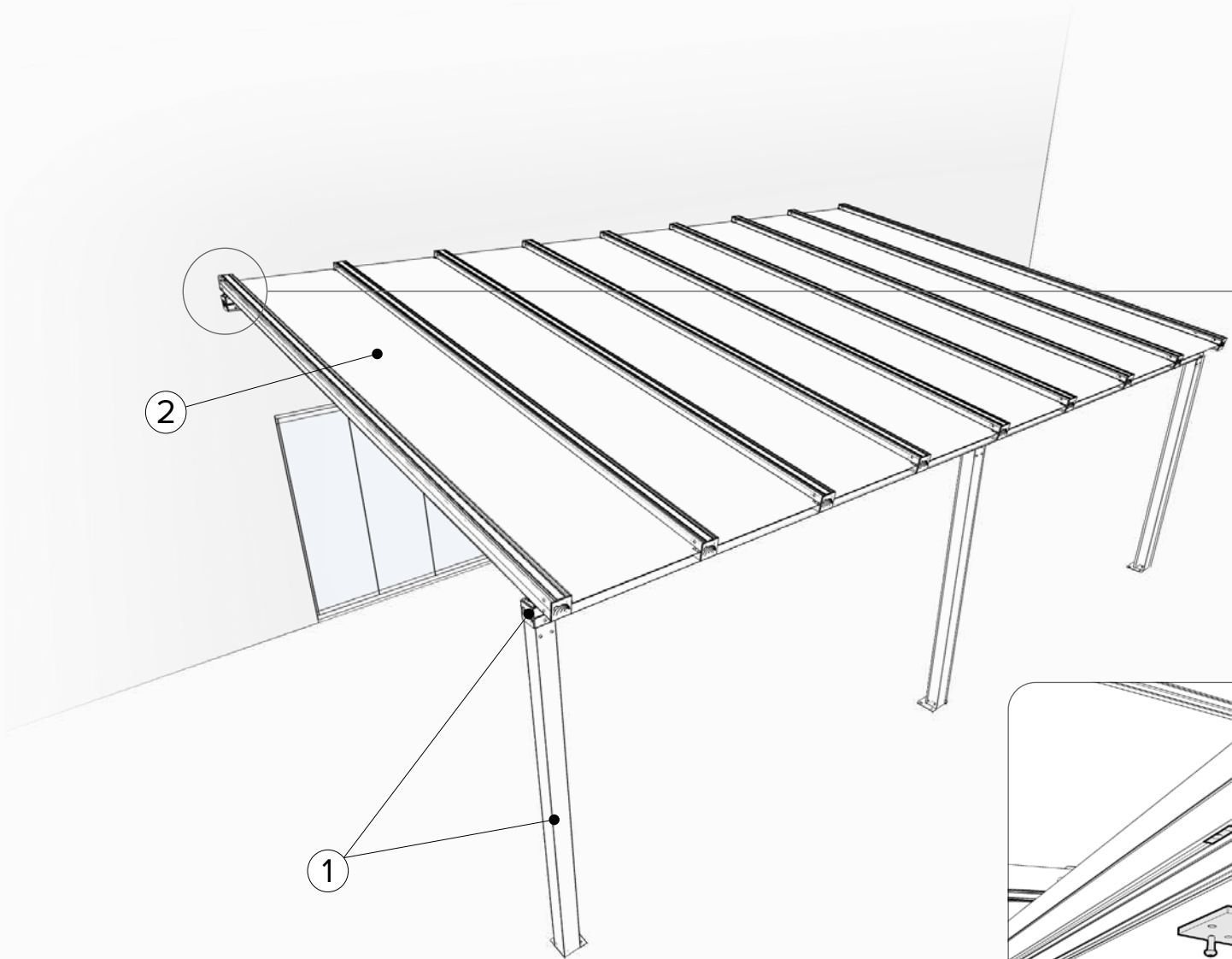
WALL-TYPE FASTENING SYSTEM
