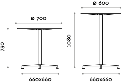
STYLO C Dimensioni base 660x660 mm / top ø 700 mm / H 730 mm
