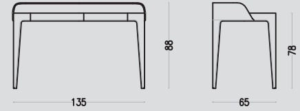
Flaminia Writing Desk Art 5051 MAAM
