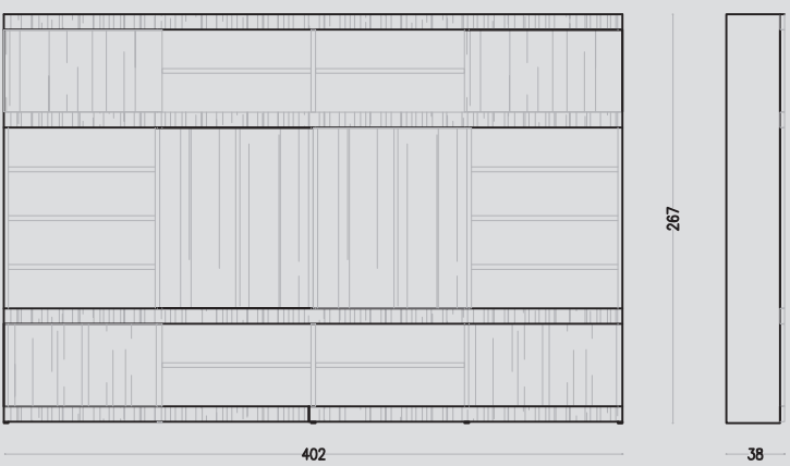
Maschera Wall Unit Sliding Doors ART FS3510597 MAAM
