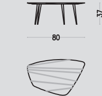
Gene Coffee Table Art 5616/A Itamar Harari
