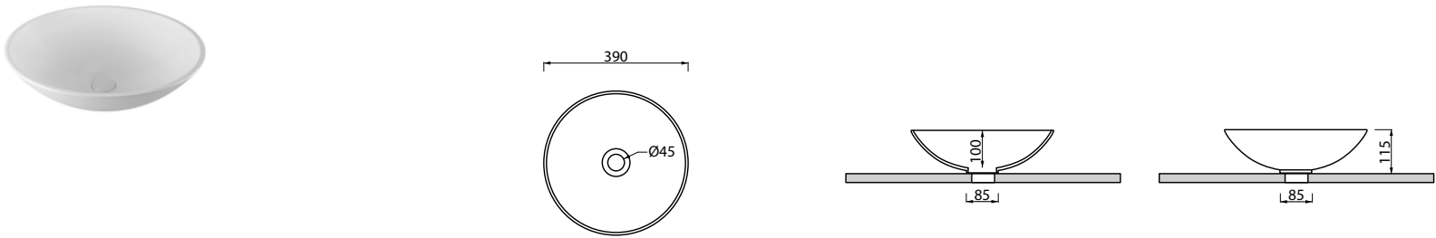
_LAVABO FLAT 7 Art. LVF7 Lavabo da appoggio diametro 39 cm senza troppopieno Laid on washbasin diameter 39 cm without overflow
