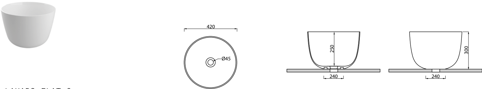
_LAVABO FLAT 9 Art. LVF9 Lavabo da appoggio diametro Ø42xh30 cm senza troppopieno Laid on washbasin diameter Ø42xh30 cm without overflow
