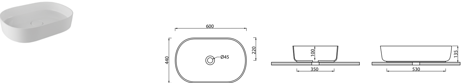
_LAVABO FLAT 8 Art. LVF8 Lavabo da appoggio 60x44 cm senza troppopieno Laid on washbasin 60x44 cm without overflow
