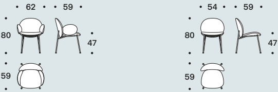
Sedia con e senza braccioli / Chair with and without armrests
