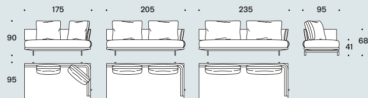
Laterali DX-SX / Right-left side units
