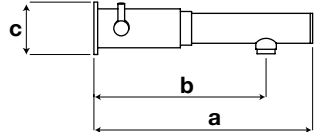
➤ Art. AB119 Miscelatore per fotocellula aria, acqua e sapone in ottone fuso lucidato e cromato per il montaggio a parete. (non idoneo per Tovel e Bisel) Polished and chromed cast brass sensor faucet for air, water and soap, wall-mounted (unsuitable for Tovel and Bisel)
