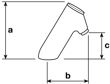
➤ Art. AB 102 Rubinetto a fotocellula in ottone fuso lucidato e cromato Polished and chromed cast brass sensor faucet
