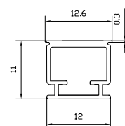
fianco destro right side
