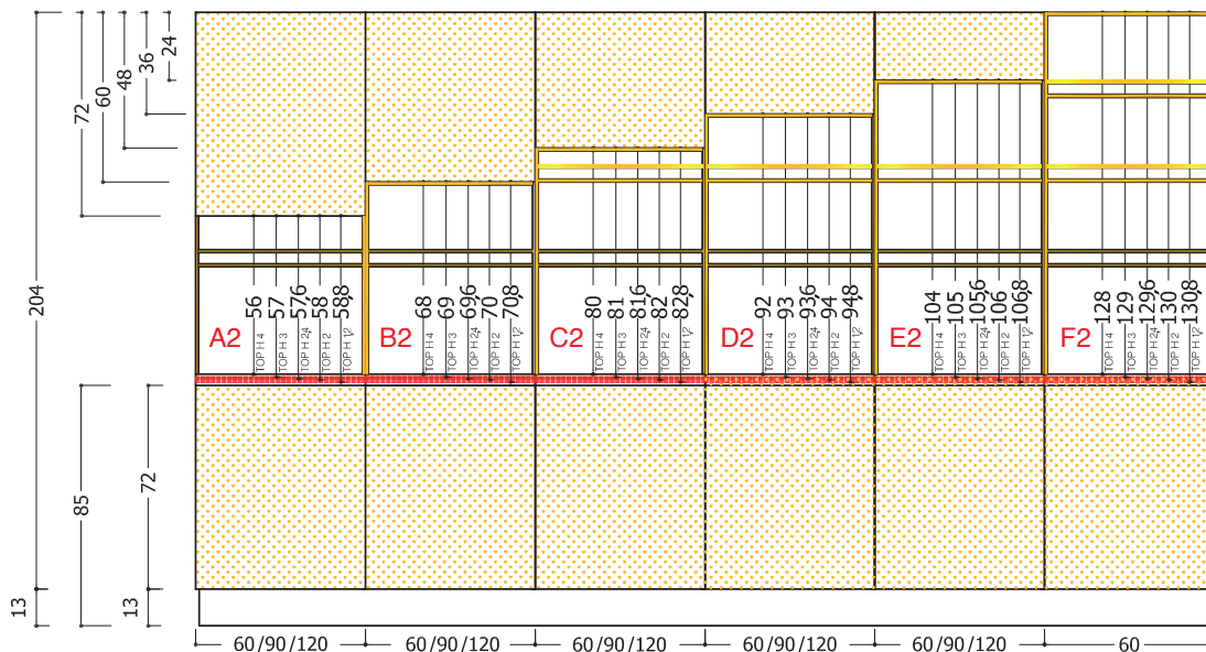
RETROTOP "MODULAR" PER BASI H.72 ZOCCOLO H.13 "MODULAR RETROTOP" FOR H 72 BASE UNITS WITH H 13 PLINTH
