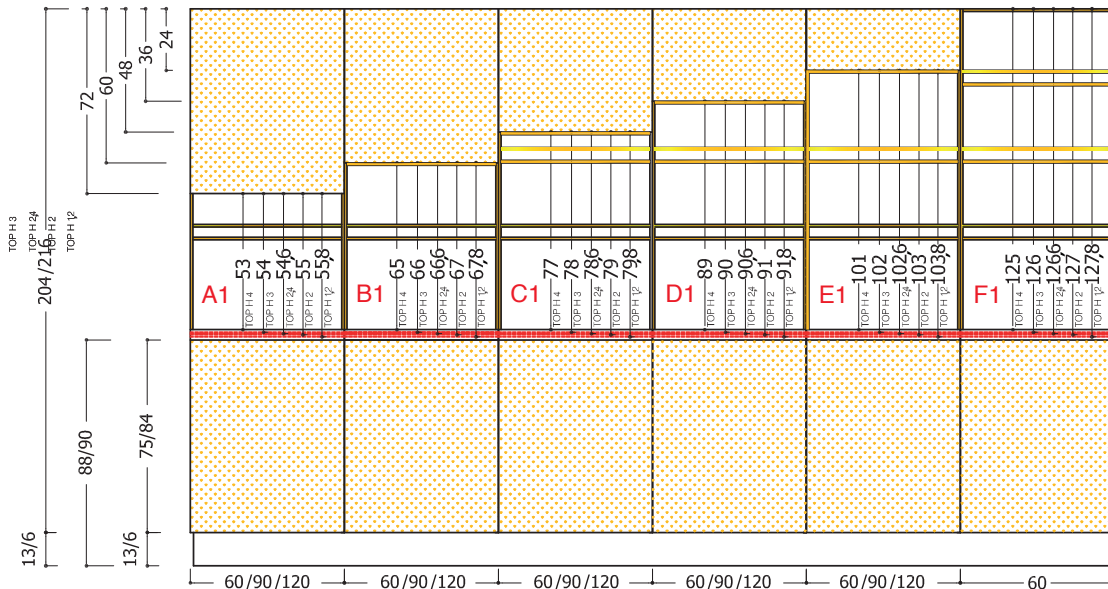
RETROTOP "MODULAR" PER BASI H.75 ZOCCOLO H.13 e BASI H. 84 ZOCCOLO H. 6 "MODULAR RETROTOP" FOR H 75 BASE UNITS WITH H 13 PLINTH AND H 84 BASE UNITS WITH H 6 PLINTH
